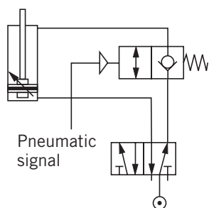
Example of Control System
