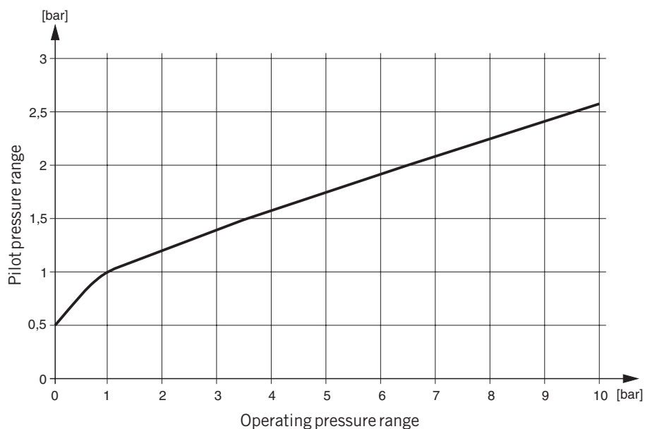
Pilot pressure in relation to operating pressure
