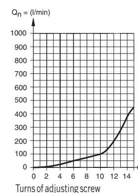
Flow characteristics Type: DV-1/4
