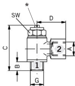
Screw-in flow control valves Type: EDV-....CI
