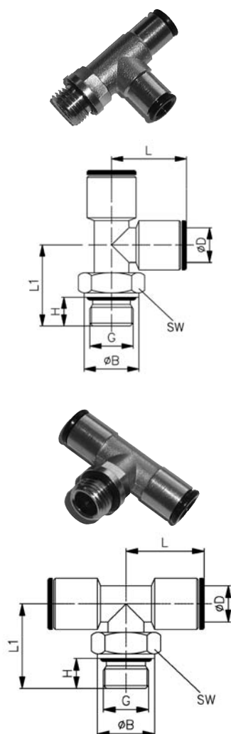
Branch tee adaptor, swivelling, male parallel thread with O-ring
