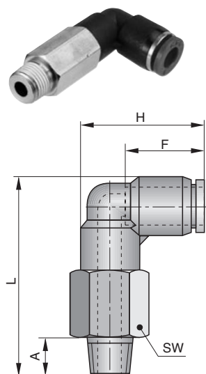
Extended elbow adaptor, swivelling, PTFE-coated male taper thread (long version)
