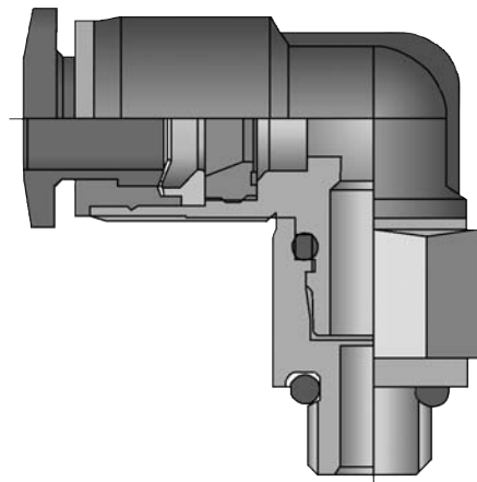
Elbow adaptor
