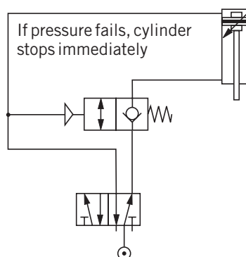
Example of Control System with Vertical Load
