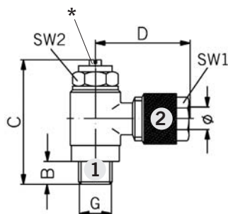
Screw-in flow control valves Type: EDV-....C
