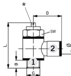
Screw-in flow control valves Type: SEDV-....C
